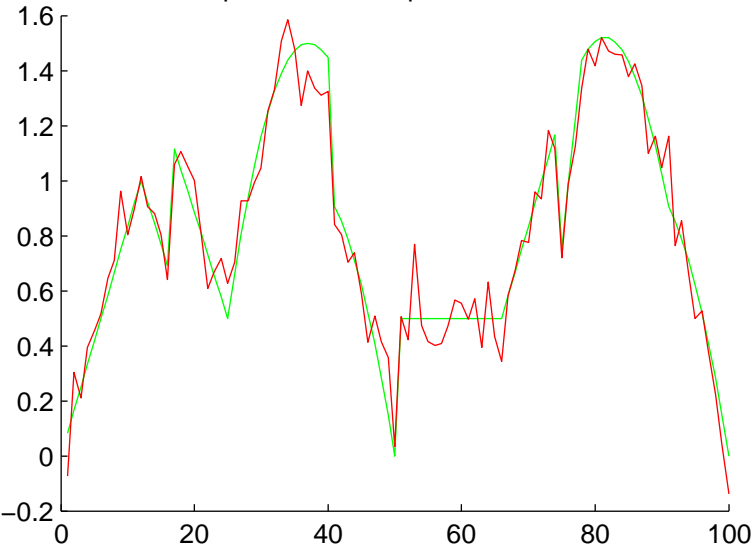
Two Sample Trials for 3-process Simulated Data
