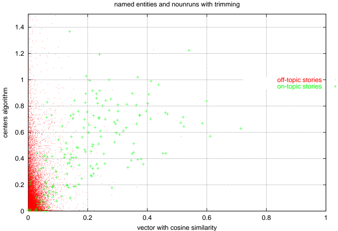
Figure 11: “Centers” algorithm gives different answers than vector with objects as features.
