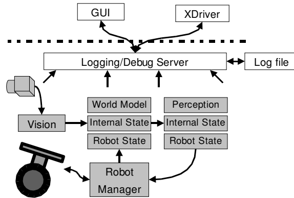
Figure 5. The control hierarchy used for the robot. The gray modules provide the system autonomy while the white modules aid in development. X-driver is a tele-operation program.
