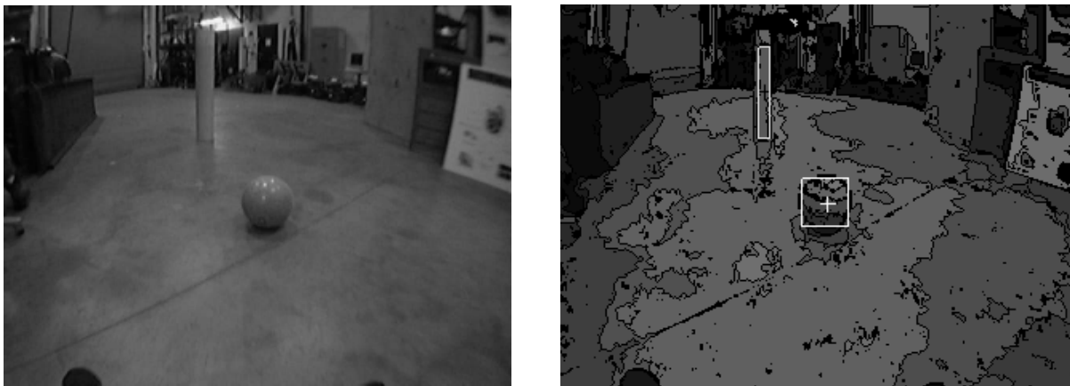
Figure 6. The left image shows a raw image in an indoor scene. The right image shows the resulting regions, with the identified ball region and yellow marker outlined with a bounding box.
