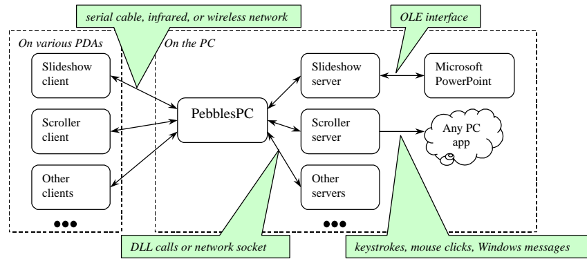
Figure 7. The Pebbles architecture.
