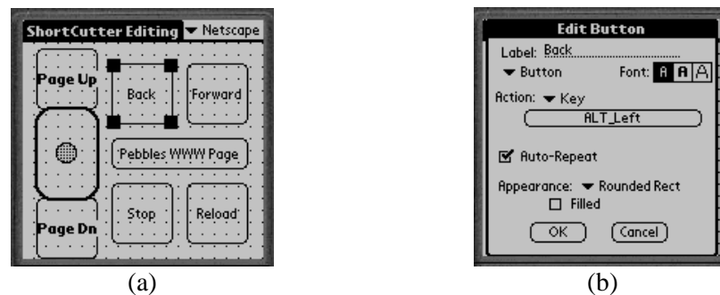
Figure 6. (a) The editing mode of Shortcutter with the Back button selected. (b) Setting the properties of the Back button so when you click on the Back button at run-time, it sends to the PC the keystroke Alt-left-arrow.
