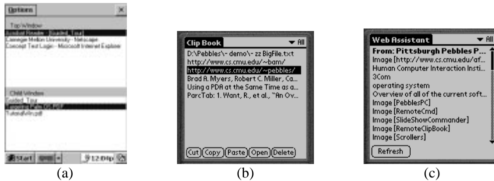
Figure 4. (a) Task Switcher displays on the PDA the top-level tasks and the windows for the selected task. (b) Remote Clipboard connects the PC’s clipboard and the PDA’s. Here is a list of items pasted from the PC, which can be copied back to the PC or to another PDA application. The “Open” button causes the selected file or URL to be opened on the PC. (c) Web Assistant displays the links on the current page. Clicking on a link causes the browser to go to that page. The list of links is only updated when the Refresh button is hit. For images that are links, the “alt” text is displayed in square brackets next to the word “Image” but if there is no “alt” text, then the URL is displayed instead.
