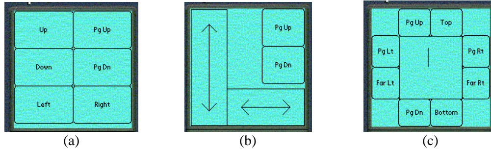
Figure 3. Three scrolling interfaces: (a) Buttons that auto-repeat to scroll up and down a line or a page, or left and right. (b) A slider, where dragging a finger or stylus in a rectangle drags the text the same amount. (c) A virtual rate-controlled joystick, where pressing in the center and moving out scrolls the text in that direction at a rate proportional to the distance.
