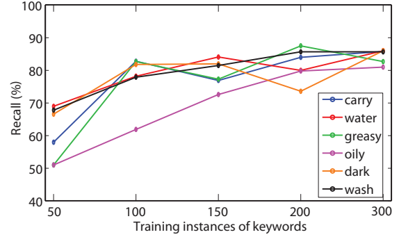
Fig. 4: Effect of increasing number of training instances of keywords for 6 different keywords.
