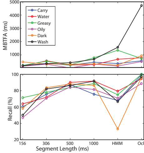
Fig. 2: Performance of forward-only gated RNN (model A), when trained with 4 segment lengths (156, 306, 500 and 1000 ms). Also shown are performance obtained with oracle segmentation (Ocl) and HMMs.
