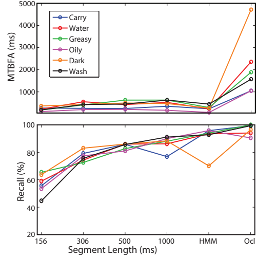
Fig. 3: Performance of Bidirectional gated RNN (model B) when trained with 4 segment lengths (156, 306, 500 and 1000 ms). Also shown are performance obtained with oracle segmentation (Ocl) and HMMs.
