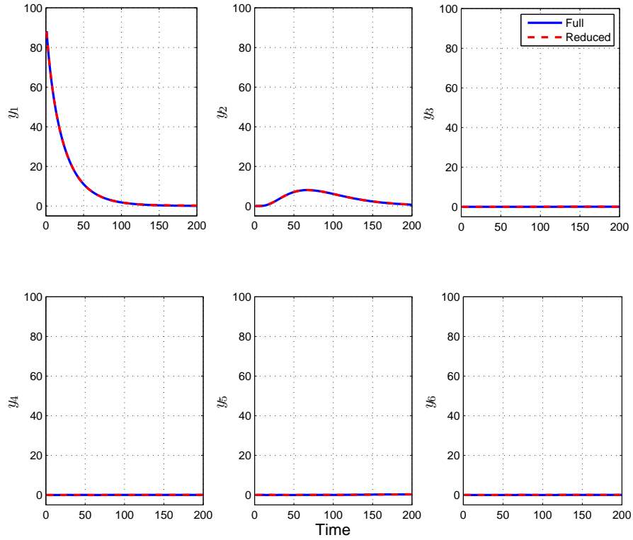
Figure 12. Full (65,600 states) and reduced (137 states) model contaminant concentration predictions at each of the six output nodes for the three-dimensional urban canyon example.
