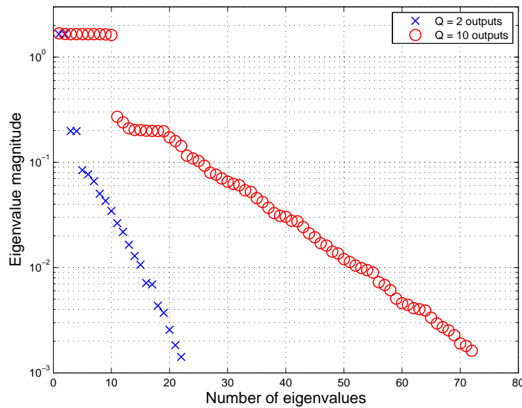
Figure 2. A comparison of the Hessian eigenvalue spectra of H for the two- and ten-output cases. Pe = 100 .
