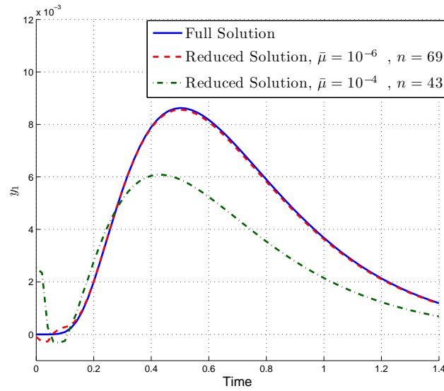
Figure 6. A comparison between full and reduced solutions at sensor location 1 for two different values of \bar{\mu} . Test initial condition (a) was used to generate the data. Pe=10 , \bar{\lambda} = 0.1 , two-sensor case.
