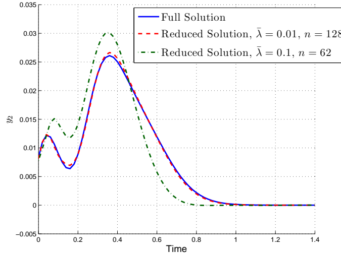
Figure 7. Lowering \bar{\lambda} to increase p , the number of Hessian eigenvector initial conditions used in basis formation, leads to more accurate reduced-order output. Test initial condition (c) was used with two output sensors, Pe=100 and \bar{\mu} = 10^{-4} . The output at the second sensor location is plotted here.
