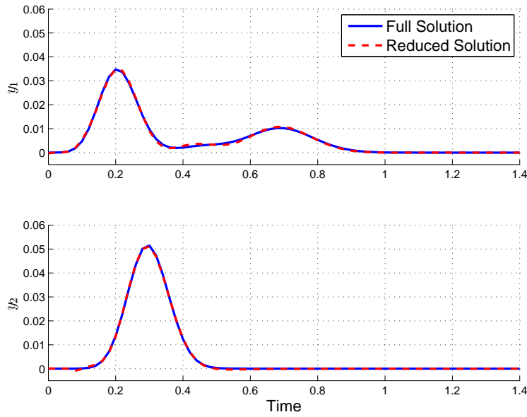
Figure 5. A comparison of full ( N = 1860 ) and reduced ( n = 196 ) outputs for two-sensor case using test initial condition (b). Pe=1000 , \bar{\lambda} = 0.01 , \bar{\mu} = 10^{-4} , \varepsilon = 0.0036 .
