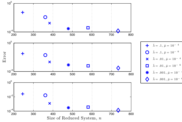
Figure 9. A measure of the error in six different reduced models of the same system plotted versus their sizes n for the ten-sensor case. The three plots were generated with test initial conditions (a), (b), and (c), respectively. Pe=100 , Q = 10 outputs.
