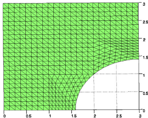
Fig. 1. Problem domain and boundary conditions for heat conduction example: Neumann on right side, Dirichlet on all other boundaries.
