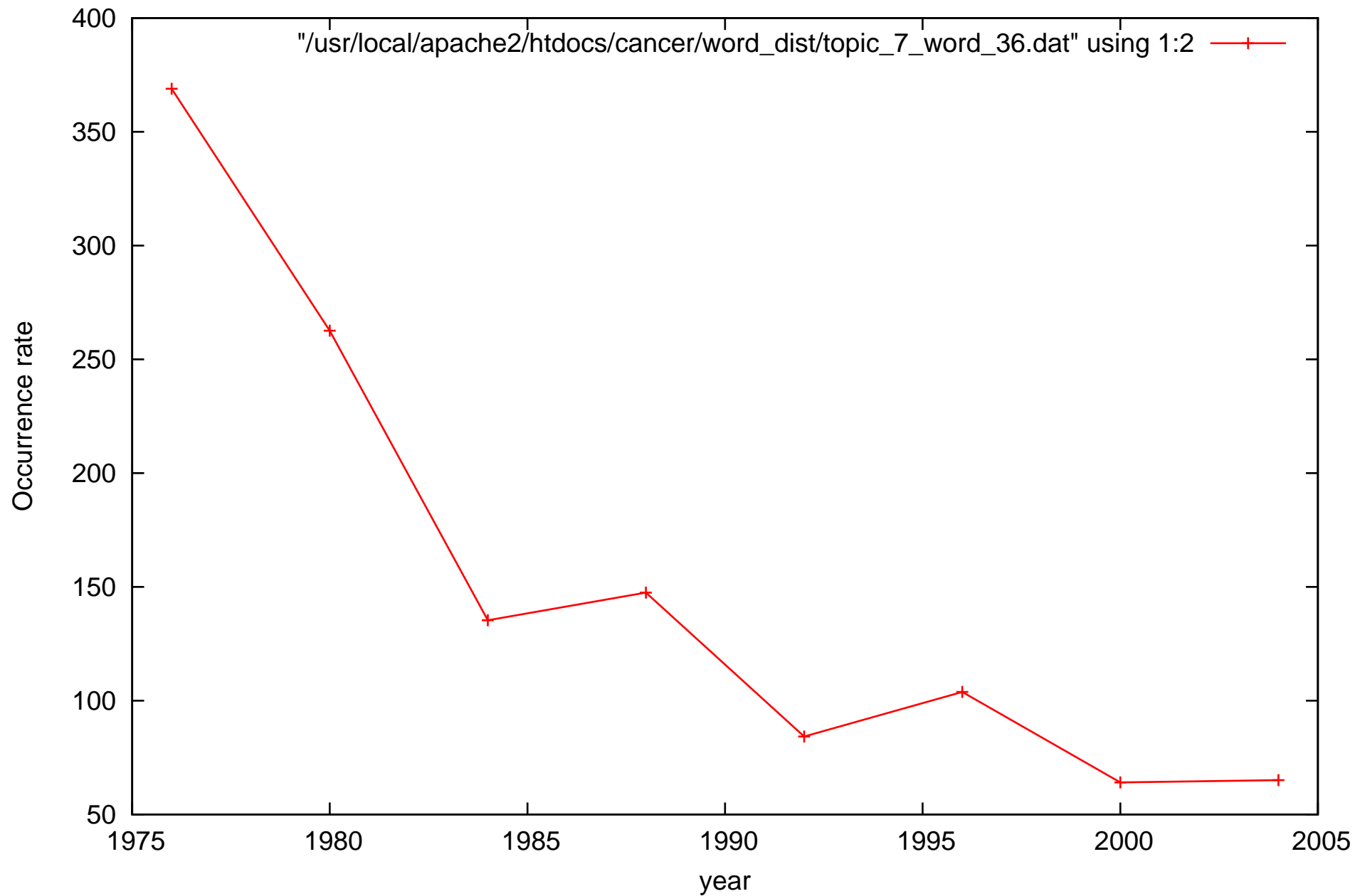
Evolution of word high in topic 7
