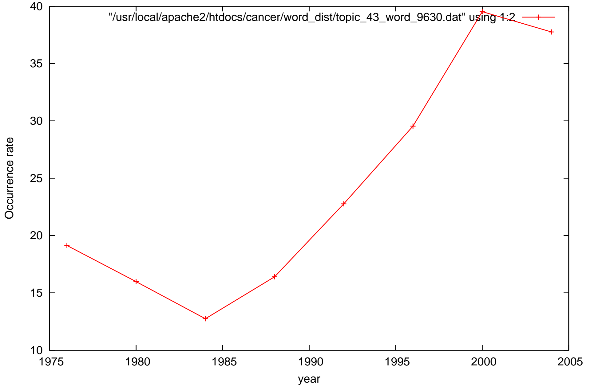
Evolution of word tool in topic 43
