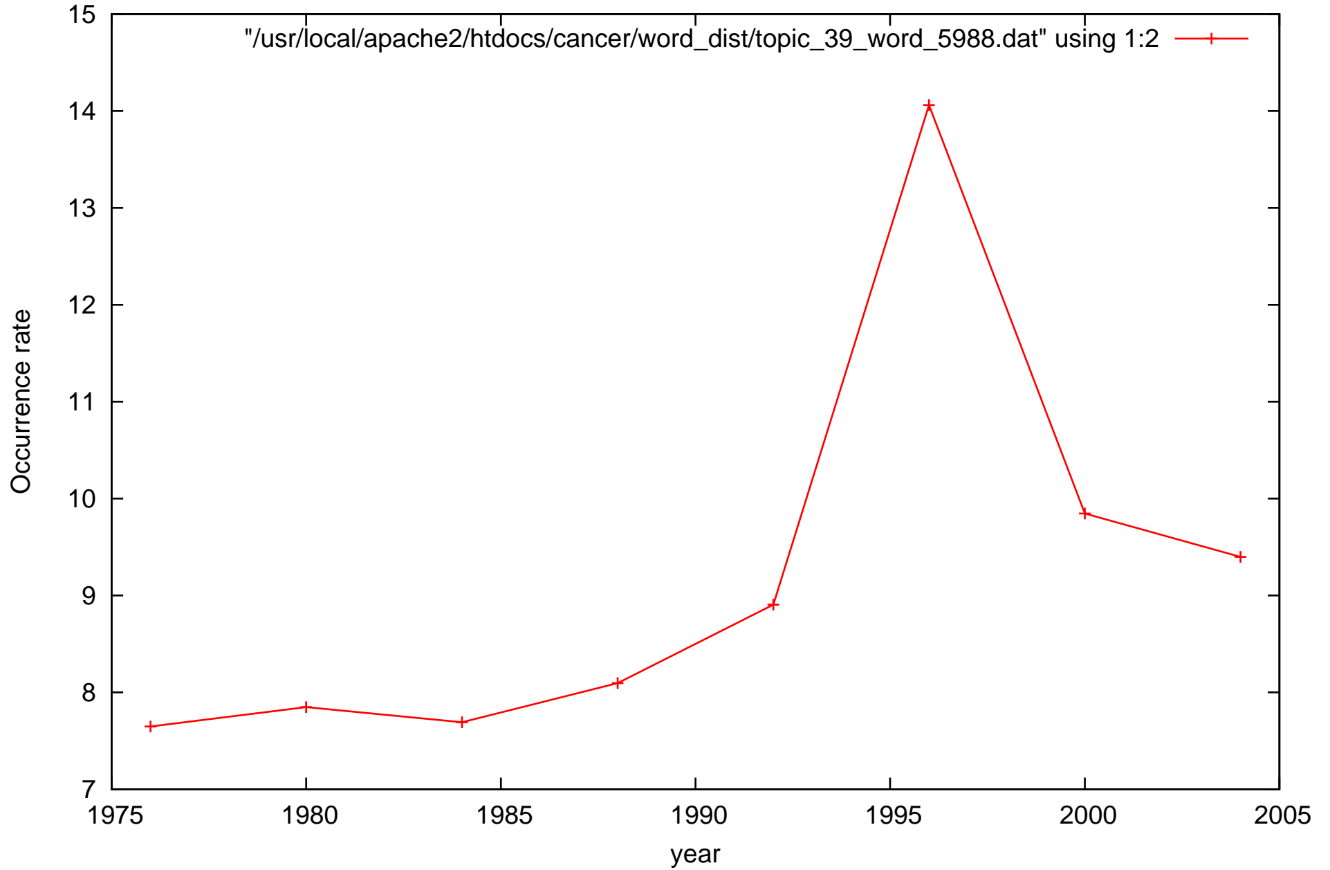
Evolution of word medicate in topic 39
