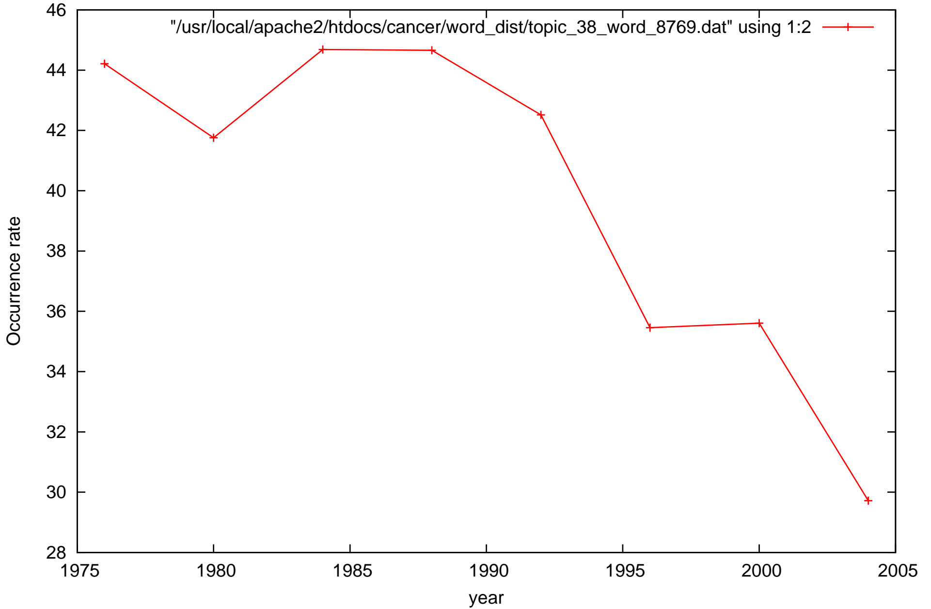
Evolution of word severe in topic 38
