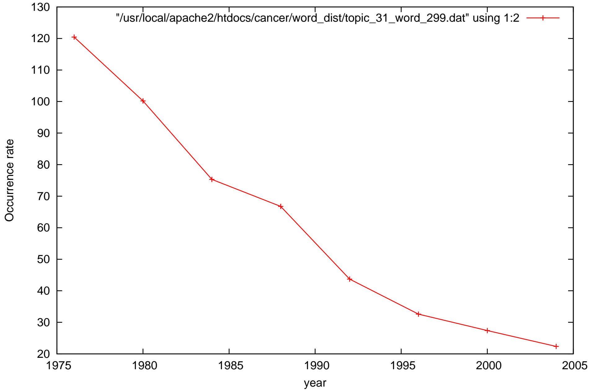
Evolution of word stomach in topic 31
