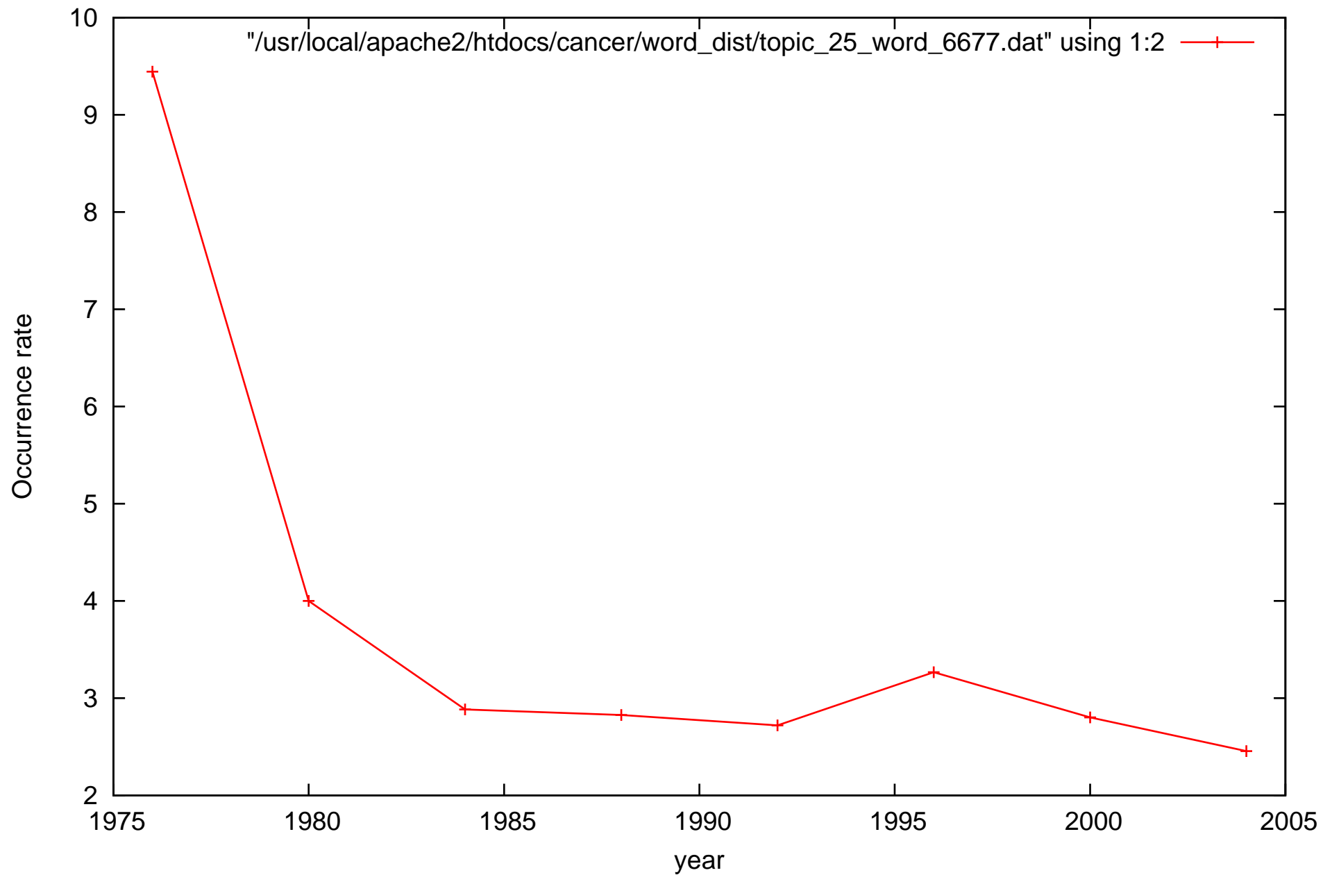
Evolution of word neutral in topic 25
