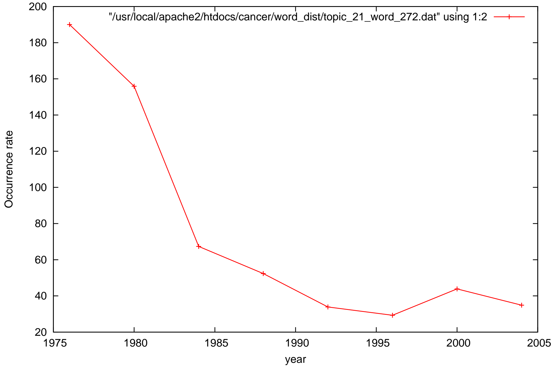
Evolution of word estrogen in topic 21
