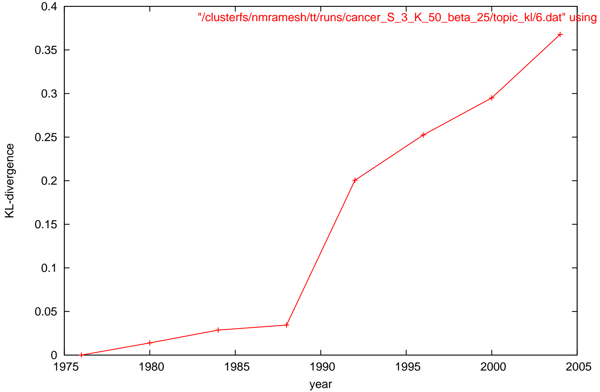
Drift of topic 6
