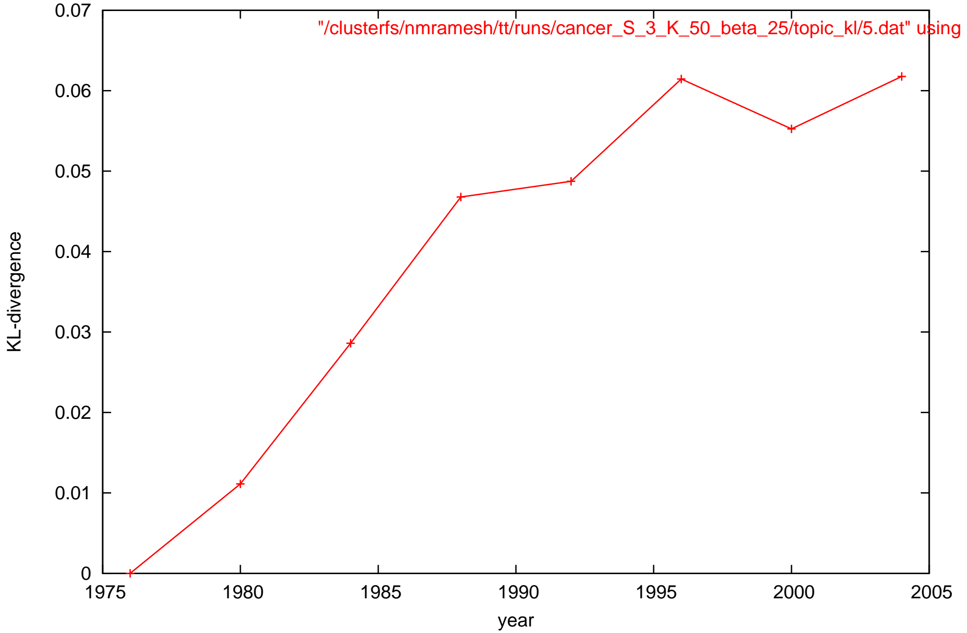
Drift of topic 5
