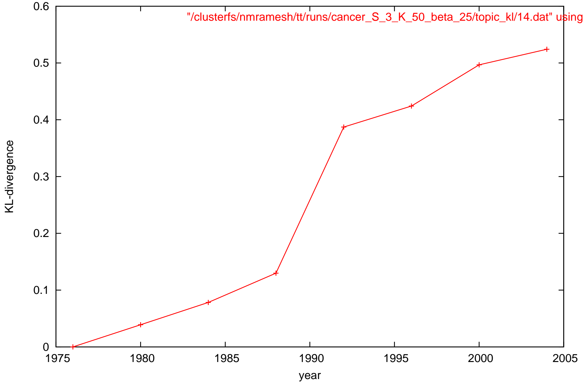
Drift of topic 14
