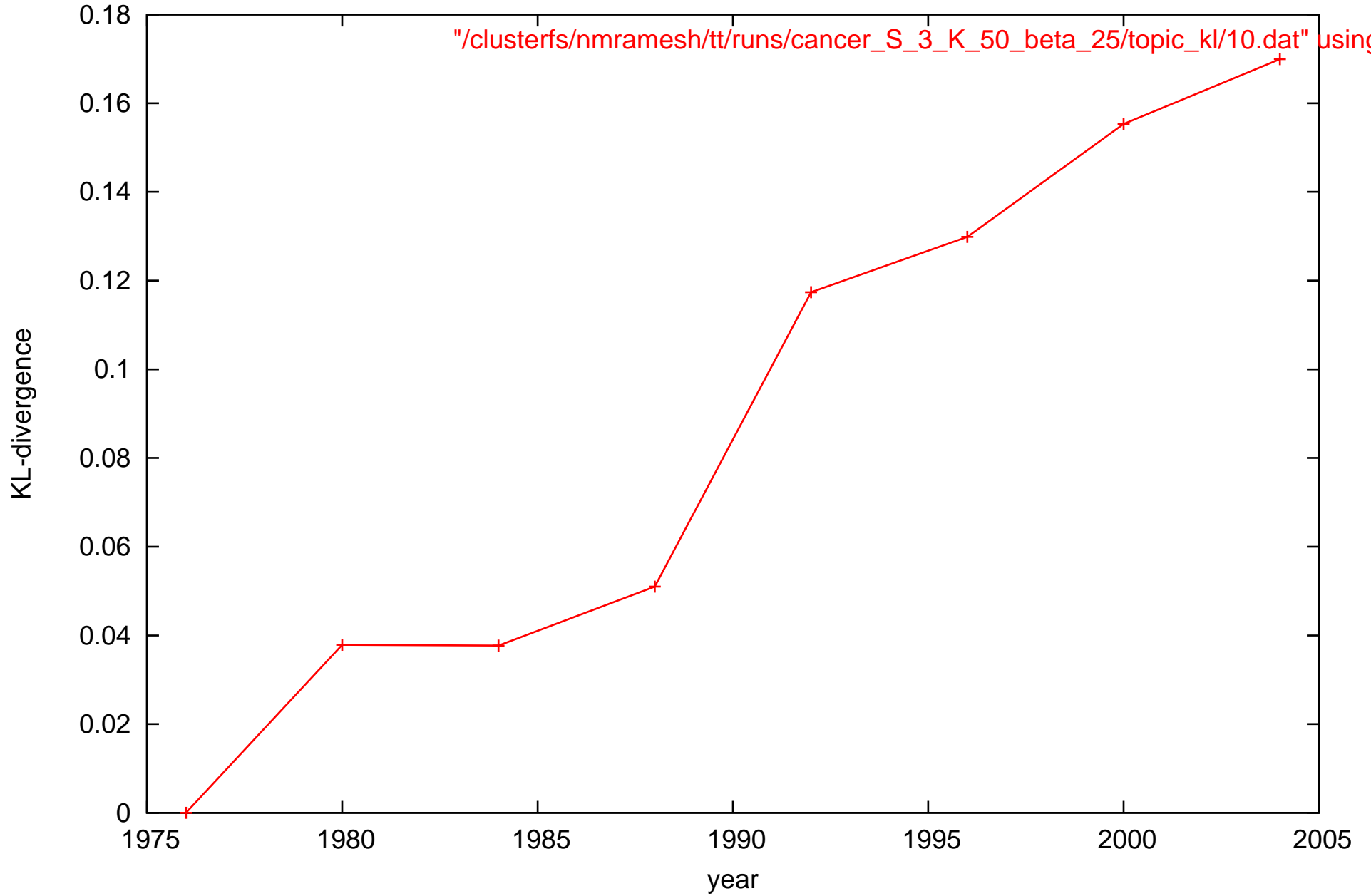
Drift of topic 10
