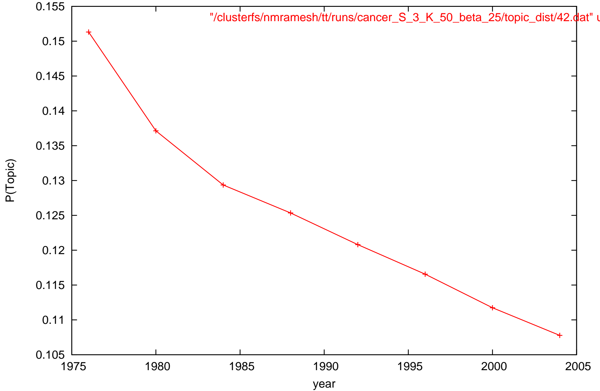
Occurrence distribution of topic 42
