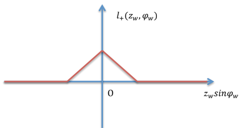
(a) l_+(z_w, \phi_w) for (normalized) hinge loss.
