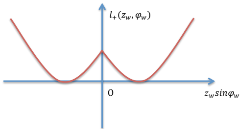
(e) l_+(z_w, \phi_w) for square loss.
