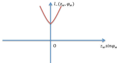
(f) l_-(z_w, \phi_w) for square loss.
