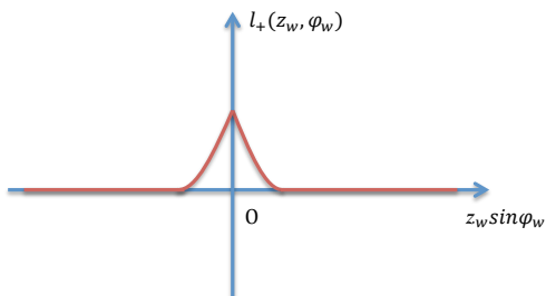
(i) l_+(z_w, \phi_w) for truncated quadratic loss.
