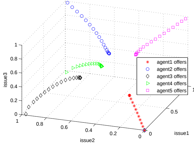
Fig. 5 Sequence of offers made by 5 agents in a three-issue negotiation scenario when agent 1 stops conceding. The agents use sequential projection along with reactive concession for generating offers. The agents come to a deadlock and no agreement is obtained although in this case the zone of agreement is non-empty (to avoid clutter, the zone of agreement is not shown here). This shows that an agent may not reach an agreement at all if she does not concede.
