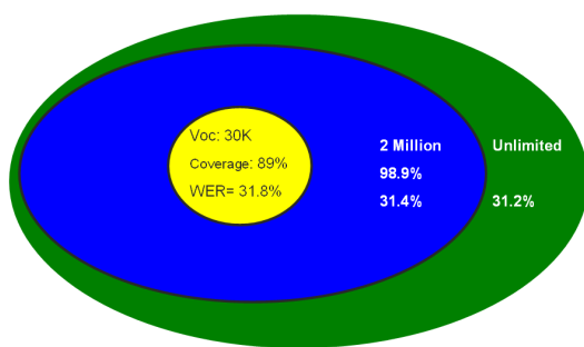
Figure 7: Correlation of Vocabulary size, Vocabulary Coverage, and WER
