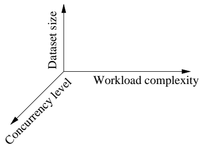
Figure 3: Benchmark-scaling dimensions.
