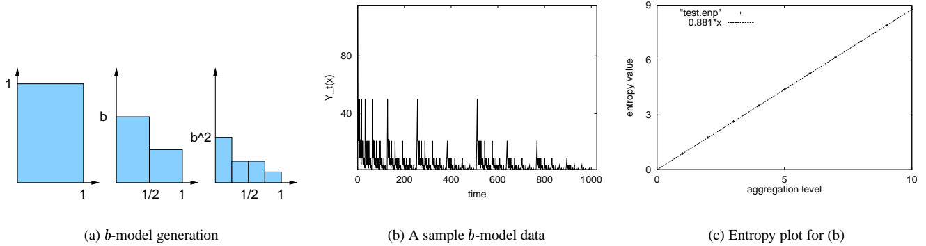
Figure 2. B-model. The sample data of bias 0.7 shows a slope of 0.881 in entropy plot.
