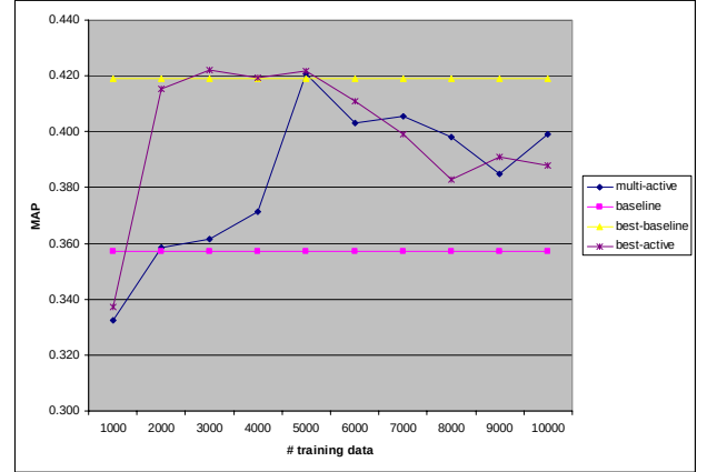
Figure 11. Classification performance for multi-modality active learning and optimal fusion approaches.
