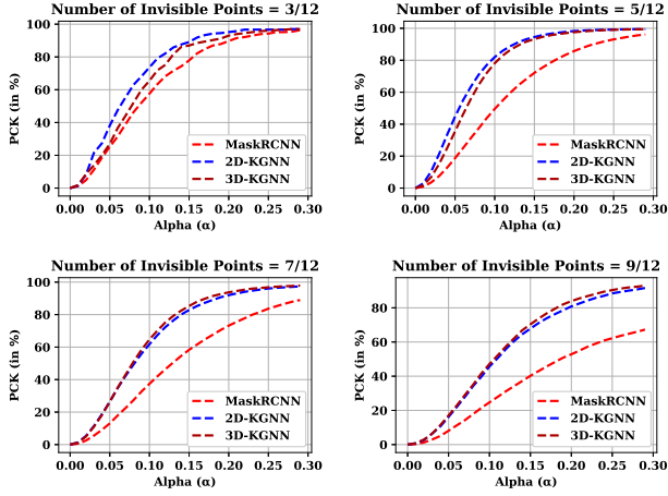
Figure 8: Accuracy vs Alpha on the CarFusion dataset. Focusing on Alpha=0.1 across the plots, graph based methods show an improvement of 6% for cases where only 3 (out of 12) points are occluded and nearly 10% or more improvement for more severe occlusion, justifying the usage of graph networks for occlusion modeling.
