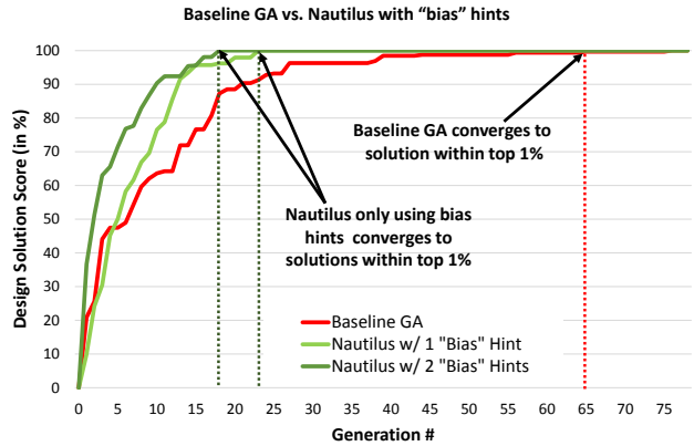
Figure 3: Baseline GA vs. Nautilus only using 1 or 2 “bias” hints.
