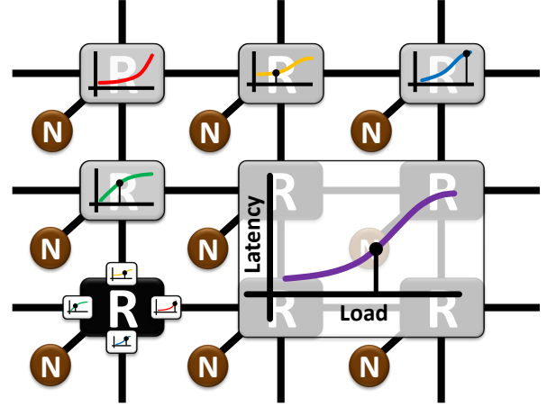
Figure 1: Representing routers as load-delay curves.
