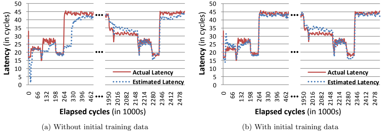
Figure 6: Actual and Estimated Latency for "LU" SPLASH-2 benchmark over a window of 3 million cycles.
