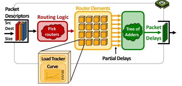
Figure 2: FIST Hardware Block Diagram.
