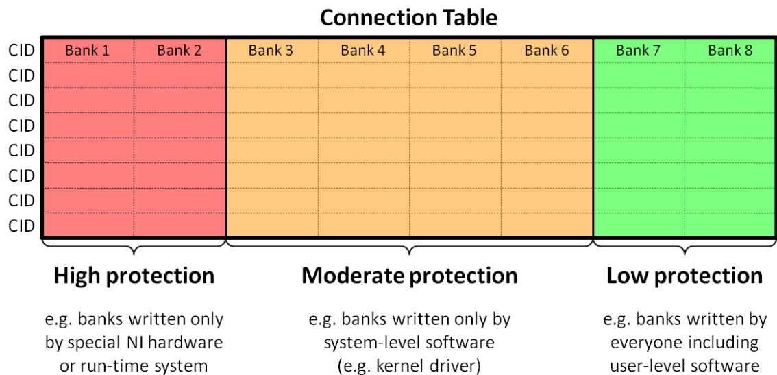
Figure 5.14 Connection Table Protection Zones
