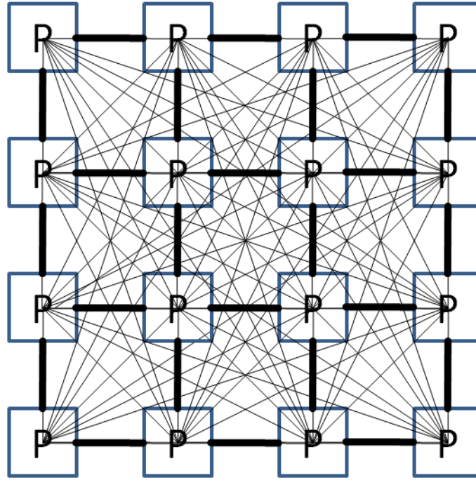
Figure 5.6: A Grid Communication Pattern.
