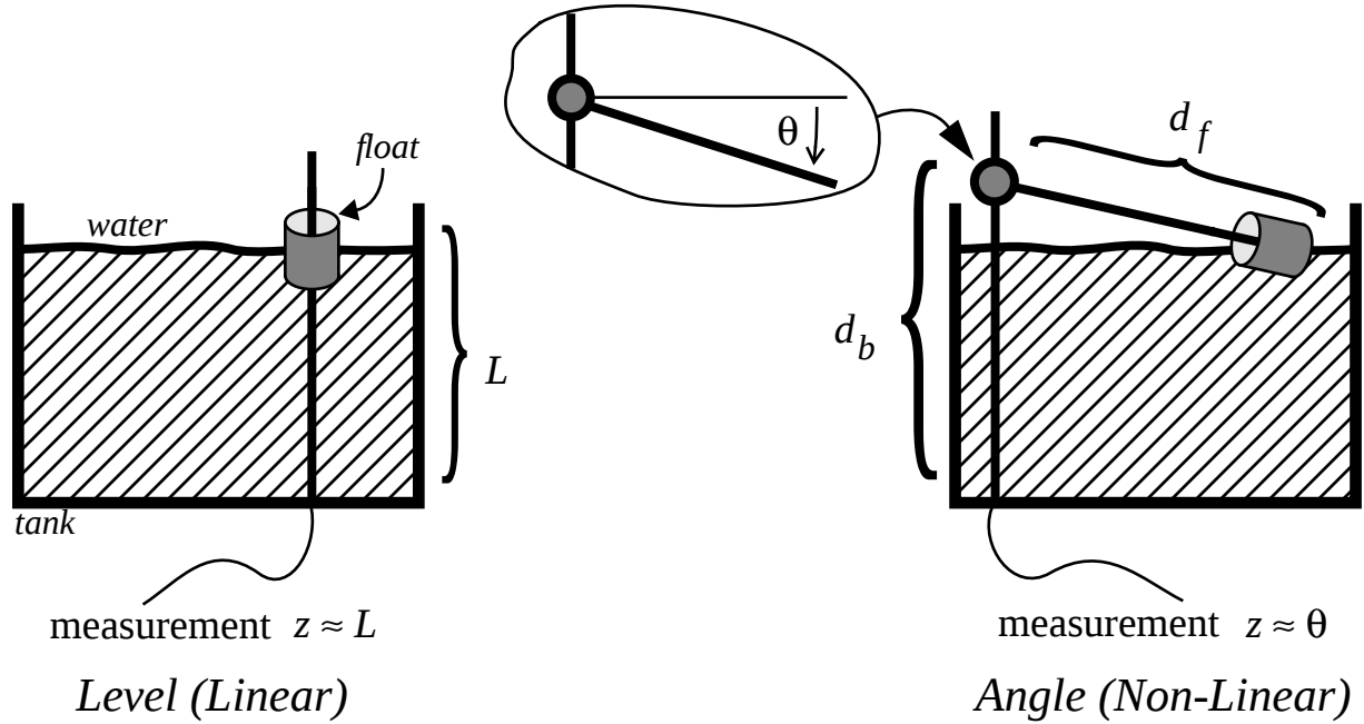
Figure 5: The two possible measurement methods. Left: the system returns a noisy voltage z representing the height of the float. Right: system returns a noisy voltage z representing the angle \theta between the fixed base segment d_b and the pivoting float segment d_f .
