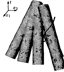
Figure 2. The configuration \times time space for Example 2. The cylinders indicate the moving obstacles in the configuration \times time space. The thick line marks the trajectory of the robot.
