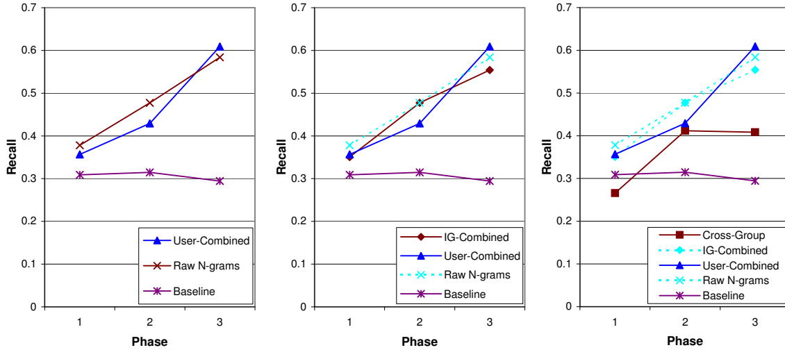
(a) Recall Values for the Final model for Individual Users comparing the Raw N-gram features with User-Combined features
