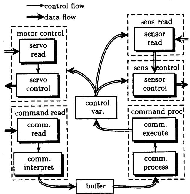
Figure 4: Robot Architecture
