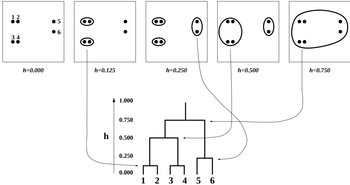
Figure 8: Example classification using numerical techniques. The top row shows how the system is clustered at several levels, parameterized by taxonomic level h ( h is distinct from information entropy H ). The classification is summarized in a taxonomic tree, or dendrogram (bottom). Strong similarities between elements are indicated by grouping near the bottom of the dendrogram; weaker similarities between groups are reflected in converging branches at higher levels.
