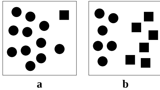
Figure 2: In both of these groups there are the same number of shapes and the same number of homogeneous subsets, but the proportion of elements in each subset is different.
