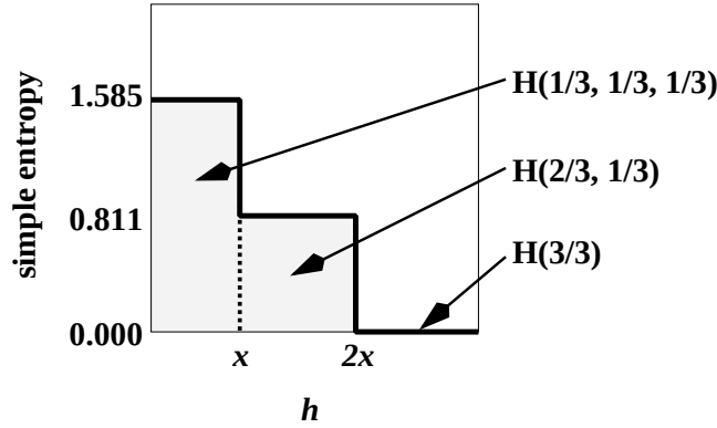
Figure 15: Simple entropy of \mathcal{R}_{2x} as a function of h . There are three distinct regions with different values.
