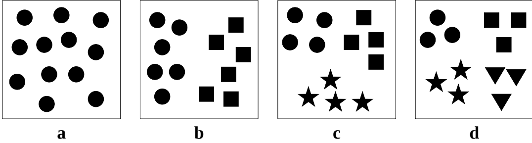
Figure 1: Several collections of shapes. The number of homogeneous subsets in each collection grows from one in a to four in d . Should measured diversity depend on the number of homogeneous subsets?
