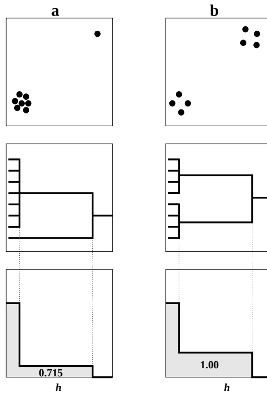
Figure 17: Hierarchic social entropy retains the basic properties of simple entropy. The computed value (bottom) depends on the distribution of elements in the subsets. Dendrograms for the two groups are also displayed (middle row).
