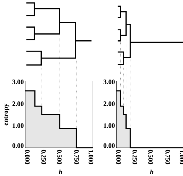
Figure 12: A comparison of entropy versus h for for two societies.
