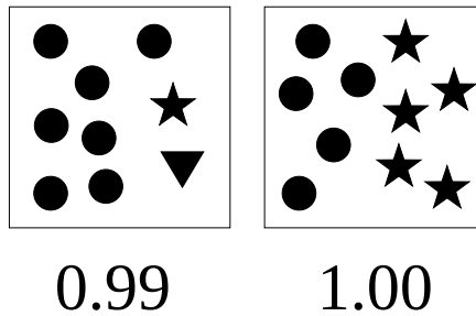
Figure 5: Two very different systems have similar entropy.
