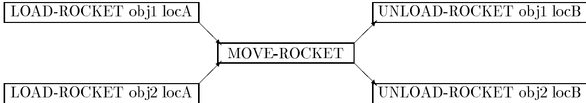
Figure 8 - Partially ordered plan for the ONE-WAY-ROCKET problem, corresponding to the four totally ordered plans consistent with the partial order.
