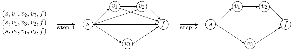
Figure 11 - Converting a complete set of total orders into one partial order.
