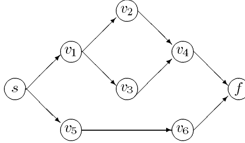
Figure 9 - An example of a partially ordered plan.
