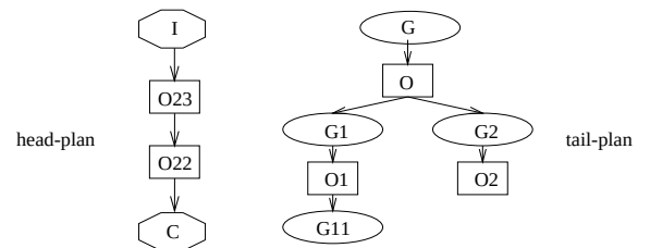
Figure 3: Representation of an incomplete plan.
