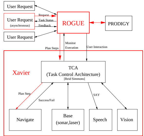
Figure 2: Rogue Architecture
