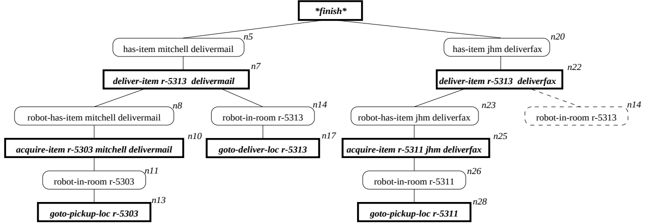
Figure 4: Search Tree for two task problem; goal nodes in ovals, required actions in rectangles.
