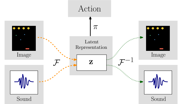
Figure 5: Summary of the three-steps approach for cross-modality transfer in reinforcement learning. The first step learns a perceptual model of the world, described by the latent mappings \mathcal{F} (and corresponding inverses), which map perceptions to a common latent space \mathcal{Z} . In the second step, the agent learns a policy \pi that maps the latent space to actions, with an RL approach using observations from a given subset of input modalities. The third step concerns the reuse of the same policy \pi , assuming new observations from a potentially different subset of modalities. This is possible by first encoding the new observations in the multimodal latent space.
