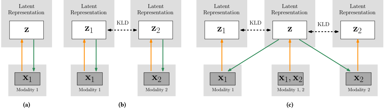
Figure 2: Networks of different generative models, highlighting the models’ data encoding (orange) and decoding (green) pipelines. The similarity constraints imposed by their training procedures are presented in dashed lines. 2a) The VAE model learns a latent representation of the data distribution of a single modality. 2b) On the other hand, the AVAE model extends the previous framework to account for multiple modalities, allowing for cross-modality inference. 2c) Finally, the JMVAE model learns a representation of both modalities, allowing for both single and joint modality reconstruction, and cross-modality inference.
