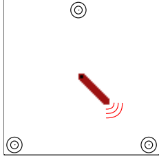
Figure 6: Visual and sound perceptual information in the PENDULUM scenario. The tip of the pendulum emits a frequency that is received by three microphones placed at the bottom left and right ( bl , br ) and middle top ( mt ).
