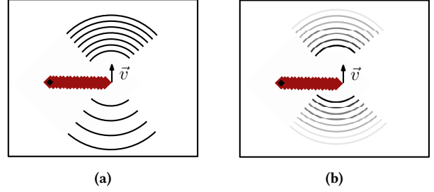
Figure 7: Different sound properties in the pendulum scenario. 7a) Depicts the Doppler effect. As the sound source moves near (away from) the observer, the arrival time of the emitted waves decreases (increases), thus increasing (decreasing) the frequency. 7b) Depicts the how the amplitude of the sound decreases with the distance from the source. Fading semi-circles denote smaller intensities.
