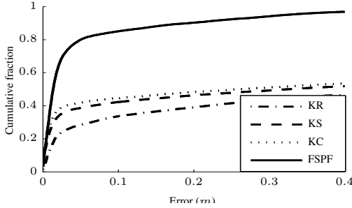
Fig. 7. Cumulative histogram of errors in localization of the different approaches. For each point (x, y) on the curves, the y value indicates the fraction of time that the algorithm had an error less than the x value.
