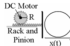
Figure 4. Rack and Pinion Kicker Schematic
