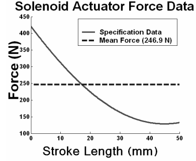
Figure 6. Solenoid Force v. Stroke and Approximation
