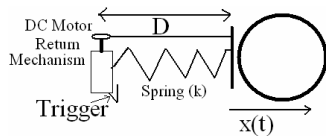
Figure 2. Spring Kicking Mechanism Schematic
