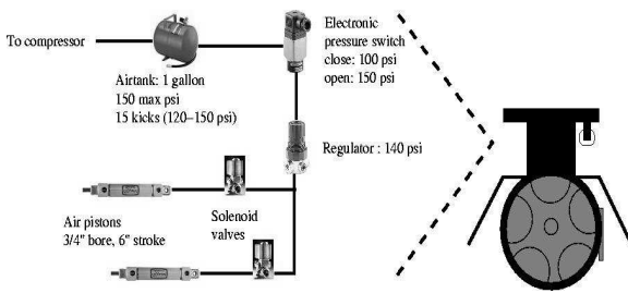
Figure 8. Schematic diagram of the implemented pneumatic kicking system
