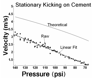
Figure 10. Stationary Kick Velocity v. Pressure
