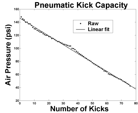
Figure 9. Number of Kicks v. Reservoir Pressure
