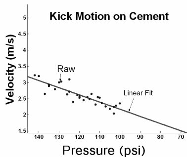
Figure 11. Kicking Motion Velocity v. Pressure
