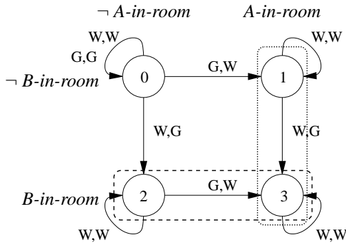
Figure 1: Doorway domain. \text{---} and \text{---} represent A's and B's goal states, \mathcal{G}_A , and \mathcal{G}_B , respectively.
