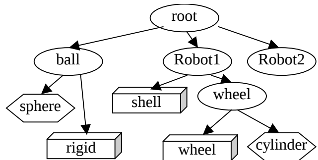
Figure 4. A simple scene graph. Rigid bodies are boxes, nodes are ovals, and hexagons are geometries.
