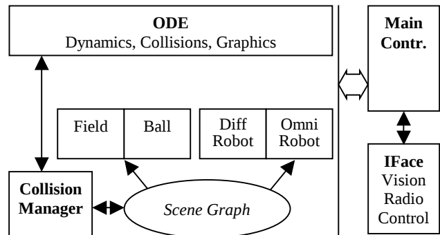
Figure 3. Major modules for ÜberSim.
