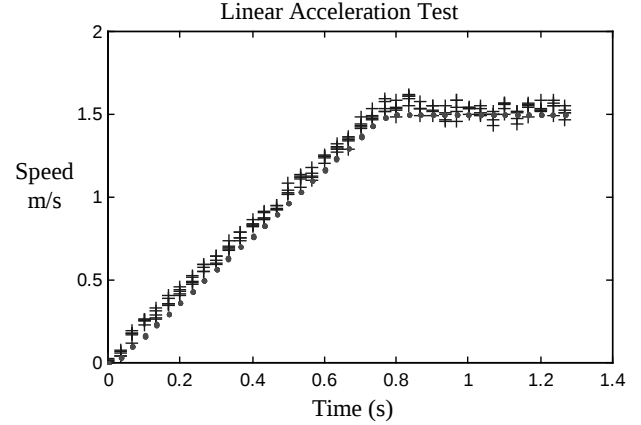
Figure 7. Acceleration comparison for a simulated Diff Robot (‘.’) versus a real robot (‘+’) repeated 5 times.
