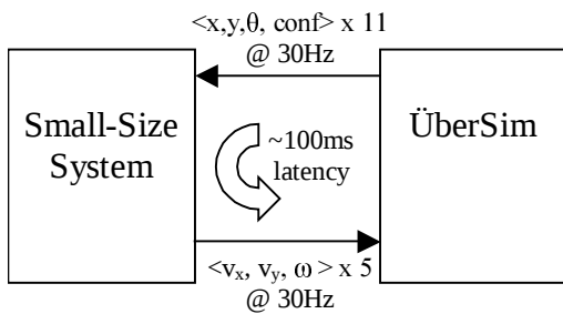
Figure 2. ÜberSim block diagram
