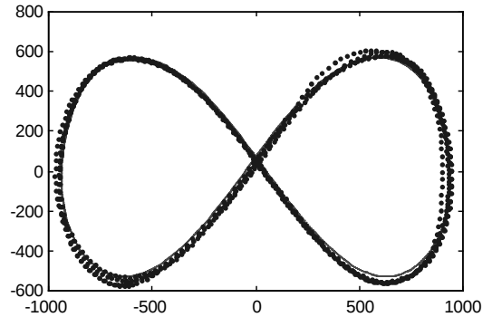
Figure 8. Trajectory comparison for simulator (line) and real robot (‘.’) performing a set figure 8 shape.
