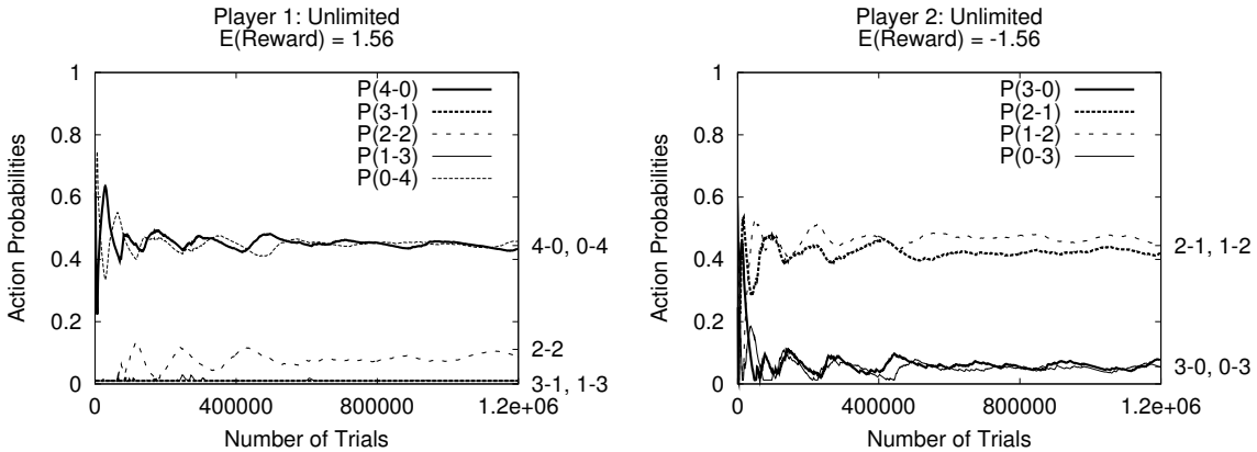
Figure 7: WoLF-PHC in Colonel Blotto. Neither player is limited.
