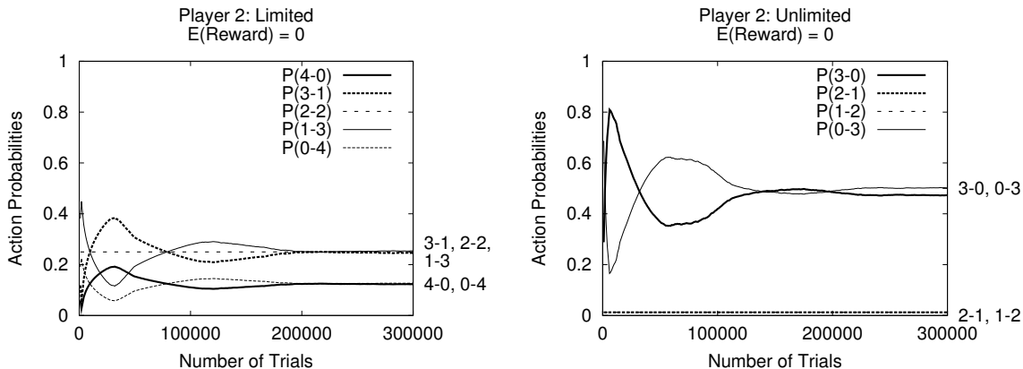
Figure 8: WoLF-PHC in Colonel Blotto. Player one is forced to randomly allot two regiments.
