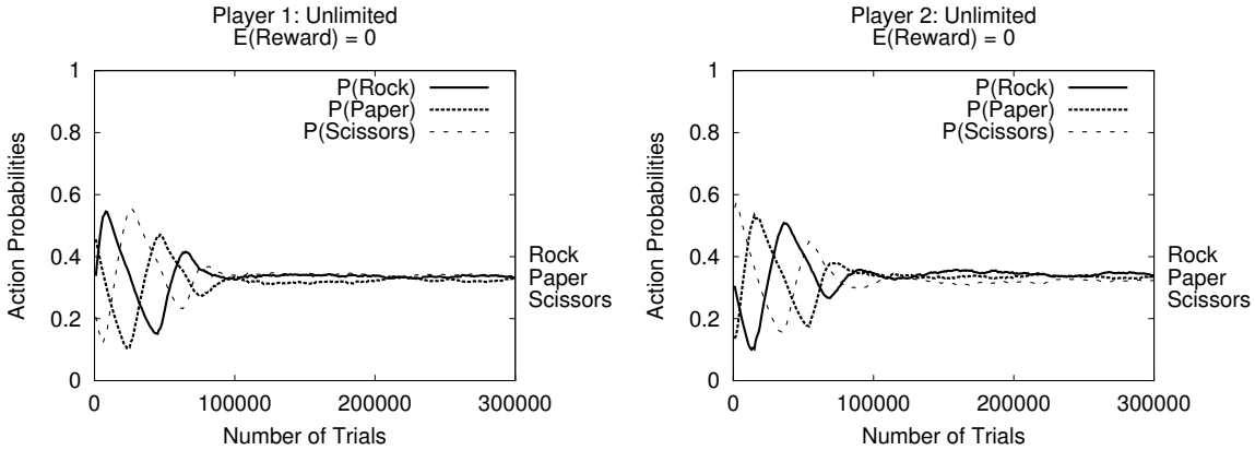
Figure 4: WoLF-PHC in Rock-Paper-Scissors. Neither player is limited.
