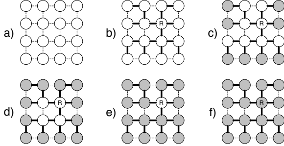
Fig. 3. Data Aggregation Algorithm: a) Available communications links b) Establishment of spanning tree rooted at R c) Leaves propagating data upwards (shaded circles) d-e) Additional levels of propagation f) Data aggregation complete
