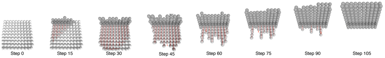
Fig. 5. Metamodule-based Shape Planner. Grey metamodules at top of structure are being created, while those at the bottom are generating deletion trees (red arrows) and being destroyed.
