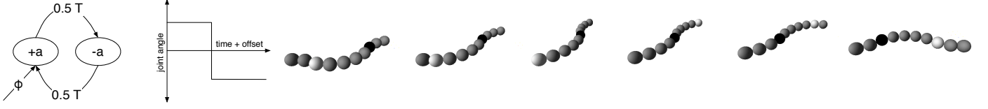
Fig. 1. a) Snake gait phase automaton, b) Joint angle vs. time graph, and c) Resulting snake gait in chain-style modules. Black modules are actuating negative joint angle, white modules are actuating a positive joint angle.
