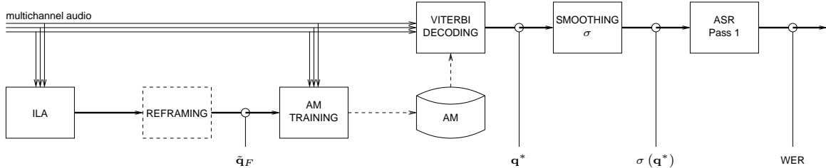
Figure 1: VAD system architecture, with 4 error measurement points. Symbols as in the text.
