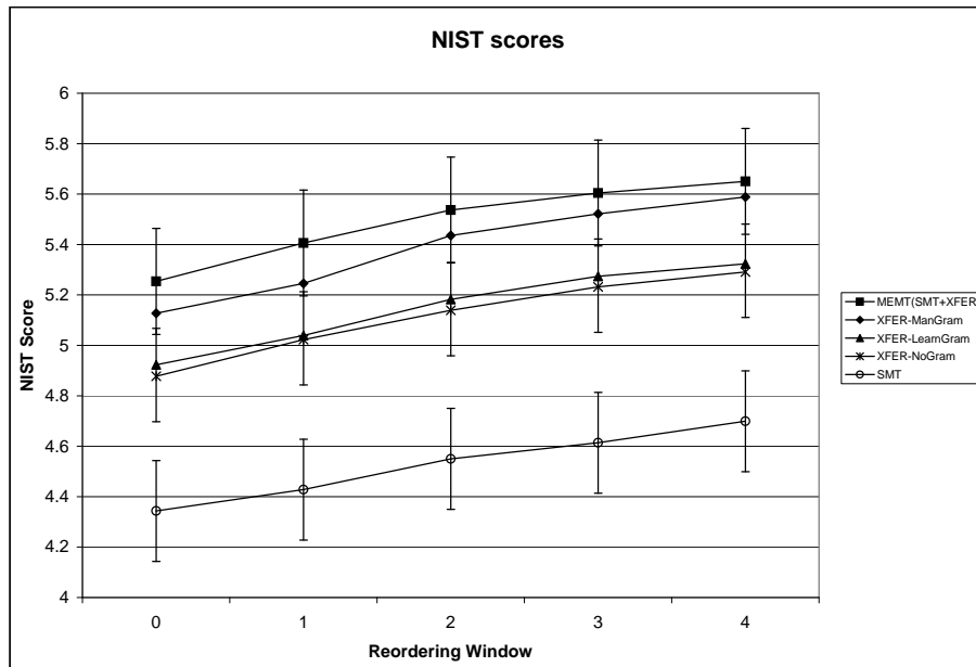
Fig. 9. Results by NIST score
