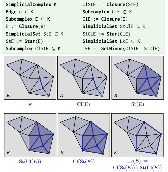
Fig. 24. A language-based specification makes it easy to visually inspect data structures or assemble progressive diagrams with only minor changes to program code. Here we draw the simplicial link by building it up from simpler constituent operations.
