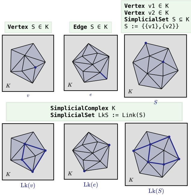
Fig. 25. Domain-specific notation makes it easy to explore an idea by trying out many different examples. Here several subsets of a simplicial complex are specified ( top ) to explore the definition of the “link” ( bottom ). An external plugin generates random example meshes, further enriching exploration.
