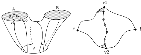
Figure 4: A Voronoi region and a Voronoi-Pair region.
