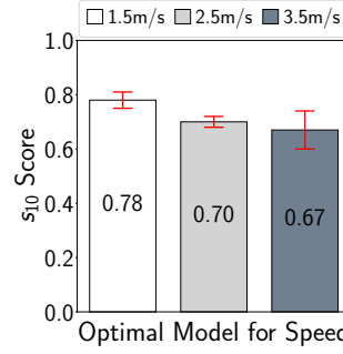
Fig. 28: Baseline Scores
