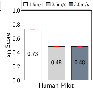
Fig. 29: Human Pilot
