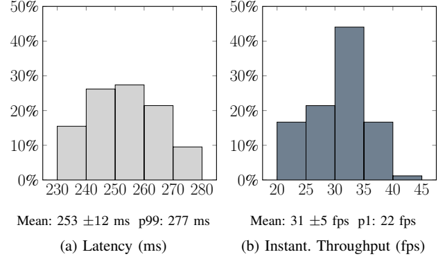
Fig. 4: Observe_{ab} Measurements
