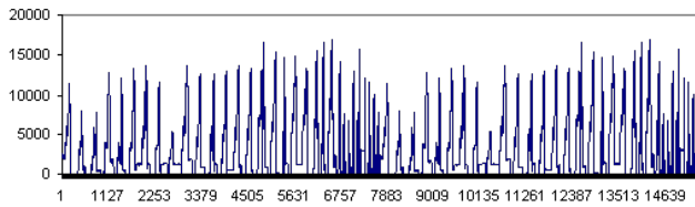
Figure 8: 1st hidden variable captures daily periodicity
