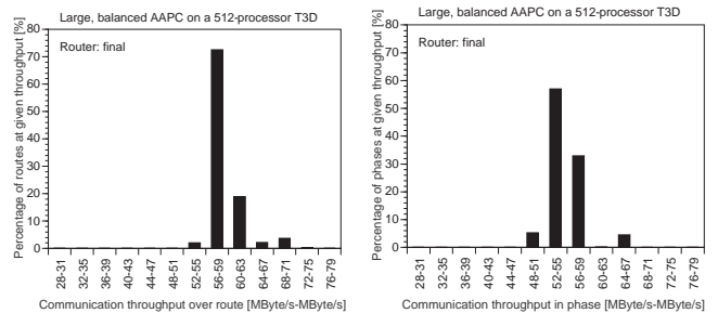
Figure 4: Histograms of transfer rates for the 512 2 routes (left), and the 512 phases (right) of a phased, machine-specific AAPC on a 512-processor T3D with a modified routing table. Each transfer is 64 kBytes.
